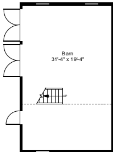
Barn - First Floor Plan Ceiling Height = 7'-8"
