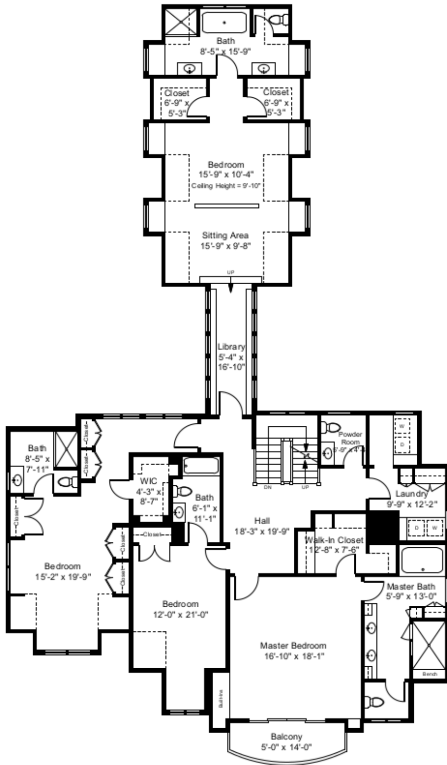
Second Floor Plan Ceiling Height = 9'-0"
