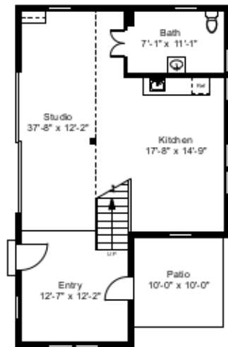
Studio - First Floor Plan Ceiling Height = 10'-5"
