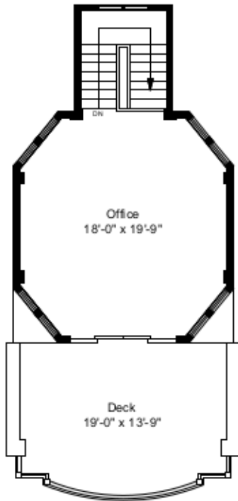
Third Floor Plan Ceiling Height = 10'-2"
